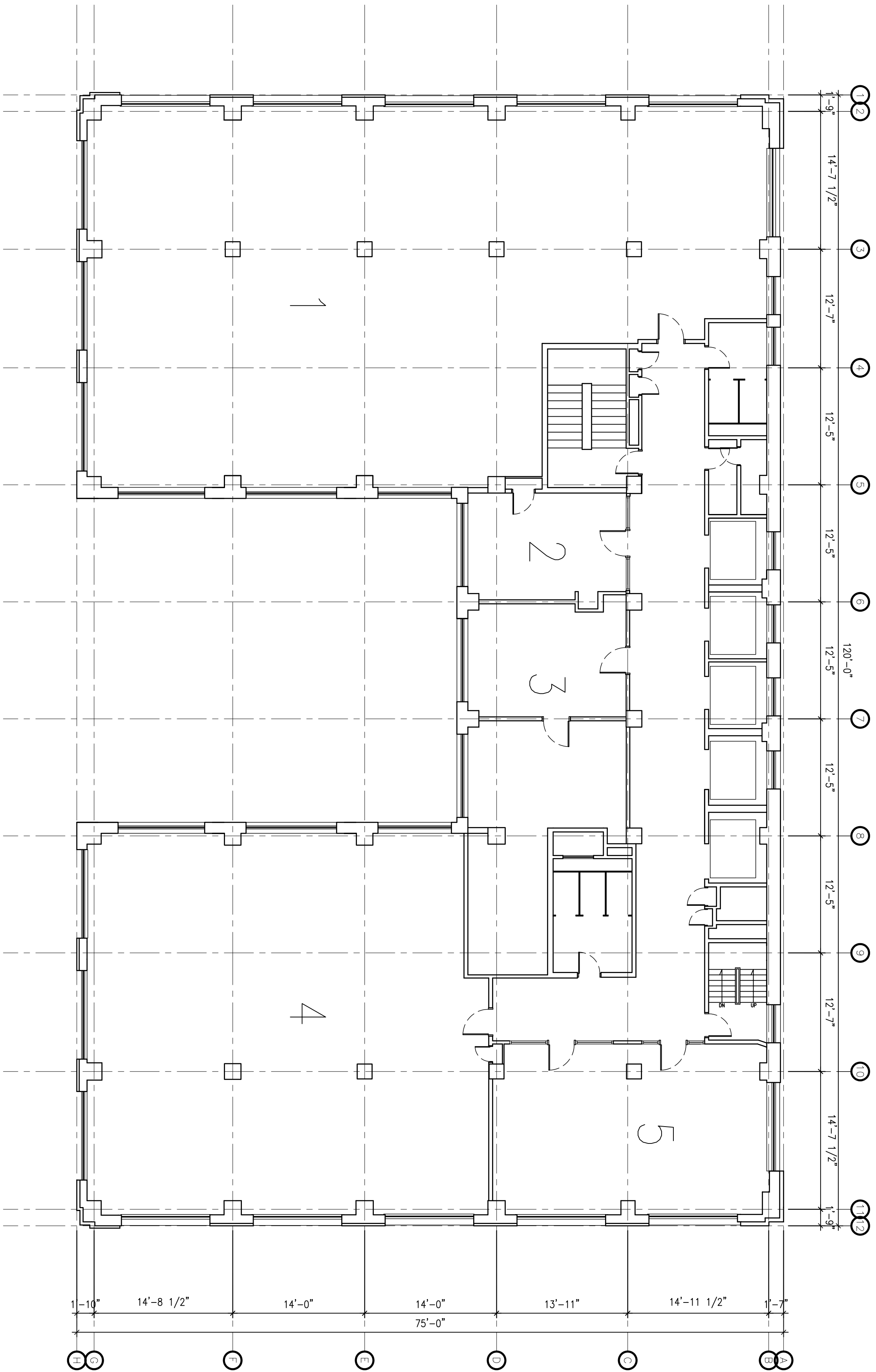
1 WASHINGTON BUILDING – NINTH FLOOR PLAN SCALE: 1/8" = 1'-0"
